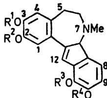
(VIII) R^1R^2 = R^3R^4 = \text{CH}_2 (XVIII) R^1 = R^2 = R^3 = R^4 = \text{Me}
