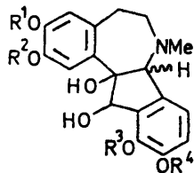
(X) R^1R^2 = R^3R^4 = \text{CH}_2 (XX) R^1 = R^2 = R^3 = R^4 = \text{Me}
