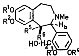
(XII) R^1R^2 = R^3R^4 = \text{CH}_2 , R^5 = \text{H} , R^6 = \text{OH} (XIII) R^1R^2 = R^3R^4 = \text{CH}_2 , R^5 = \text{OH} , R^6 = \text{H} (XXI) R^1 = R^2 = R^3 = R^4 = \text{Me} , R^5 = \text{OH} , R^6 = \text{H}_a (XXII) R^1 = R^2 = R^3 = R^4 = \text{Me} , R^5 = \text{H}_a , R^6 = \text{OH} (XXIII) R^1 = R^2 = R^3 = R^4 = \text{Me} , R^5R^6 = \text{O}
