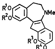
(IX) R^1R^2 = R^3R^4 = \text{CH}_2 (XIX) R^1 = R^2 = R^3 = R^4 = \text{Me}
